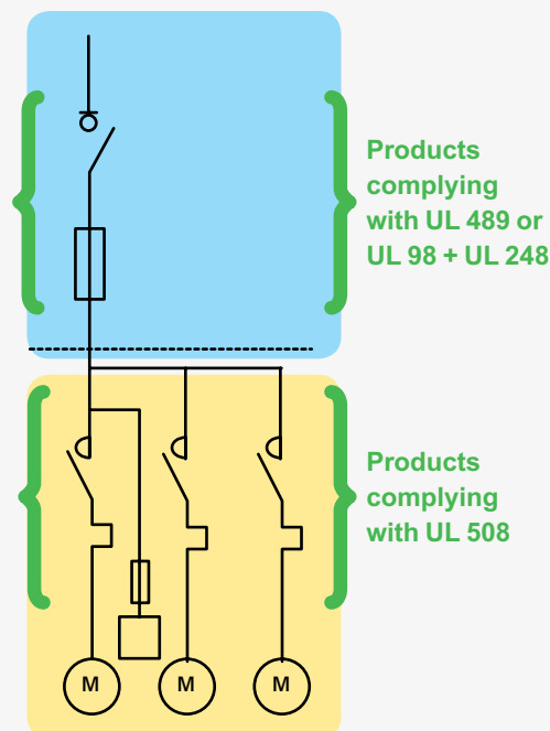
Branch circuit
