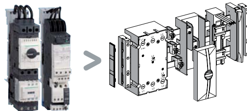
TeSys LA9Z for TeSys U and GV2: supports, busbars, terminal blocks, etc.
